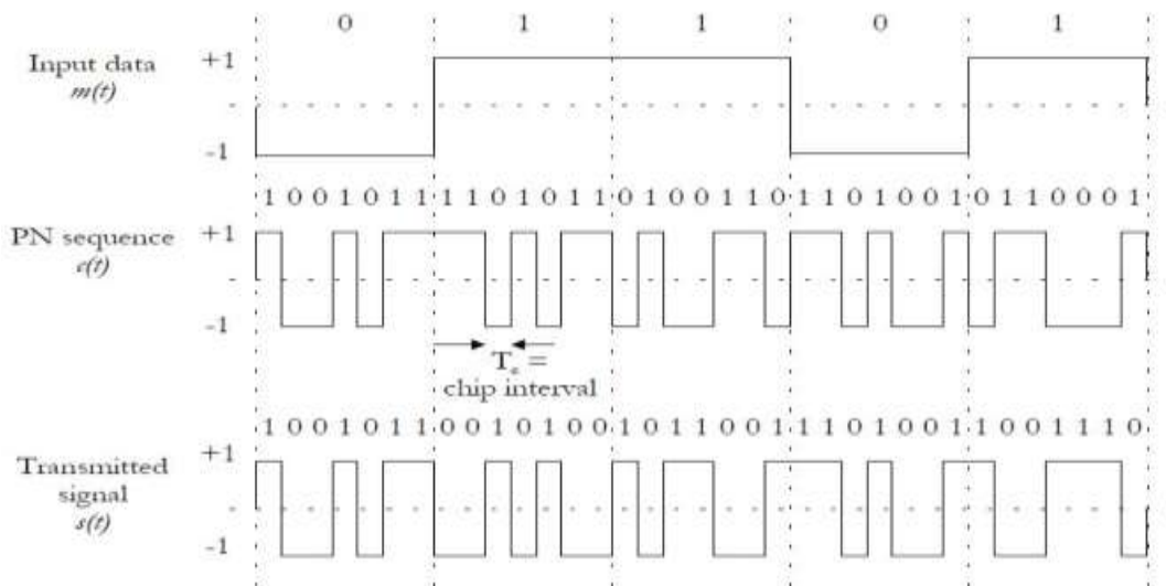
Fig -2: Generation of a DS-SS signal by using an exclusive-OR (XOR) operation.
