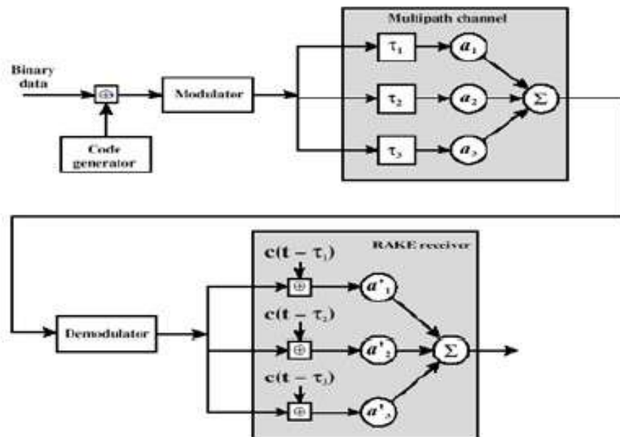
Fig -5: Block diagram of RAKE Receiver
