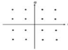
Fig – 16-QAM Constellation
