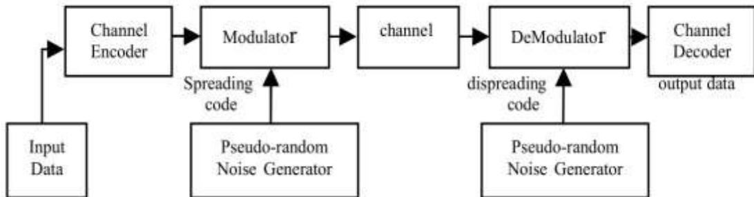
Fig -1: General implementation model of the DS-SS communications system
